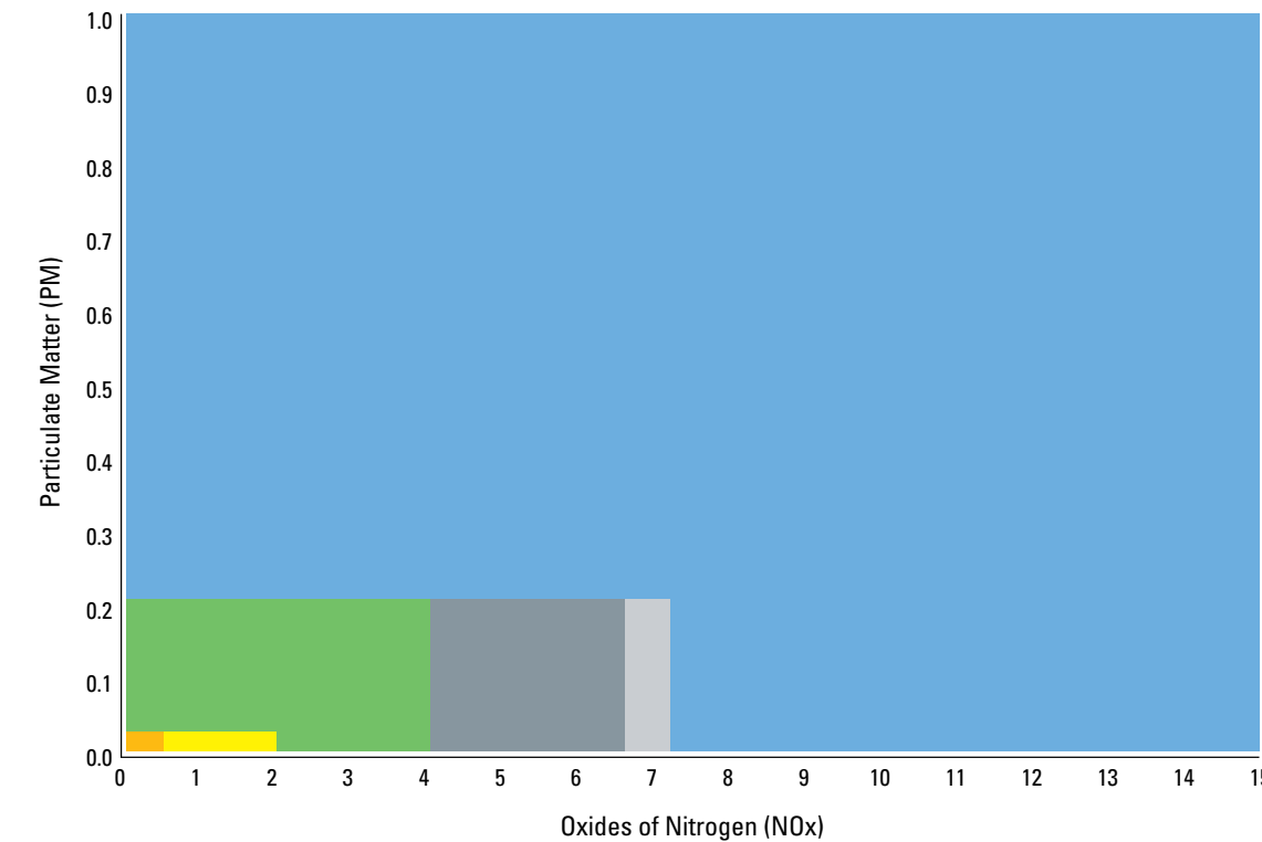
Tier 1/Stage I (1996) – Tier 4 Final/Stage IV (2014) Engines rated 130–560 kW (175–750 bhp)*
